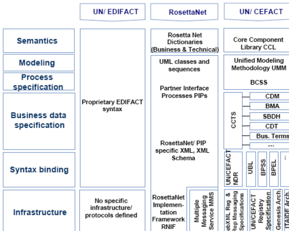
Fig. 15. UN/CEFACT e-Business stack compared to EDI and Rosetta e-Business stacks. (Source: Barbara Flügge, Till Jannerand, Christoph Schroth, SAP AG/RESEARCH Lab, St Gallen. “Technology Push vs. Market Pull. Software Engineering Companies: Corporate Research Units as Pull Facilitators” – In: EuroMOT2006 Second European Conference on Management of Technology 10th to 12th September 2006 Birmingham, United Kingdom )
